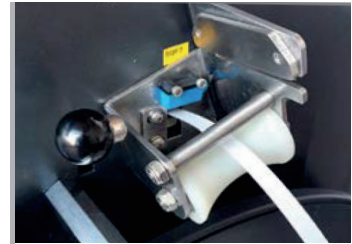
Automatic strap feeding strap cutter
