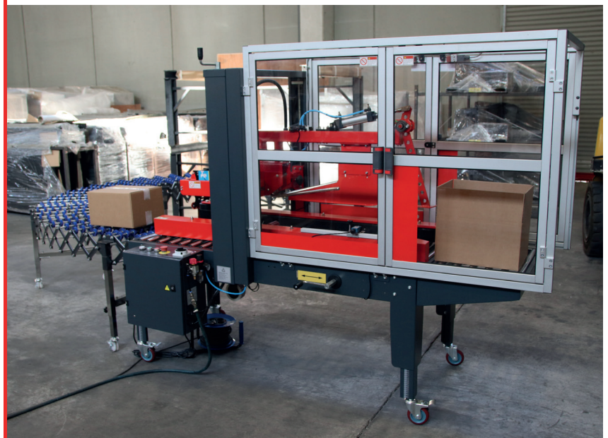
iP35 with roller carriage
